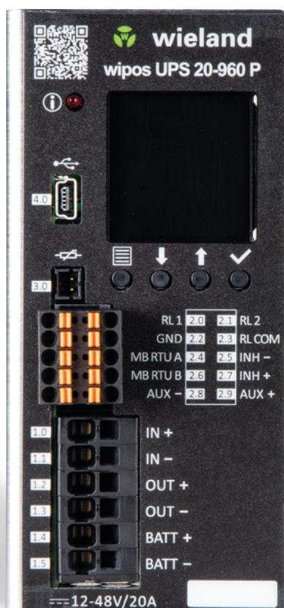
wipos UPS 20-960 P Parameterization via Display/4 control buttons and/or via wipos PLAN software
