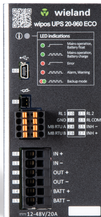
wipos UPS 20-960 ECO Parameterization only via wipos PLAN software
