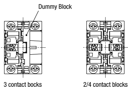
3 contact blocks
