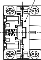
2/4 contact blocks
