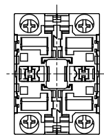
3 contact blocks
